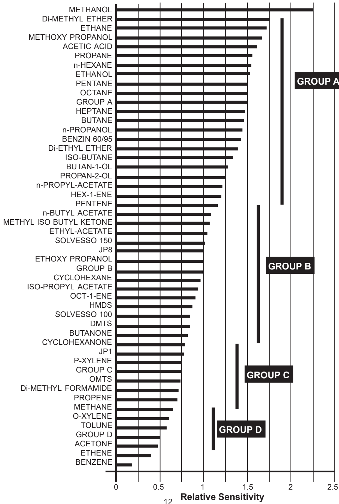
Chart 1 Relative Response Chart Relative to 'Band B' at 50% LEL
