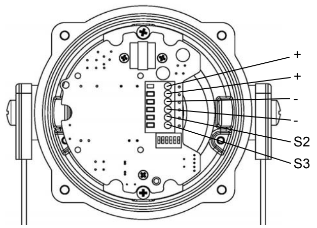
Fig. 7a Chamber LED Beacon DC Terminals
