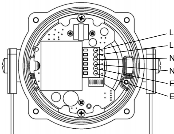
Fig. 5a Chamber LED Beacon AC Terminals
