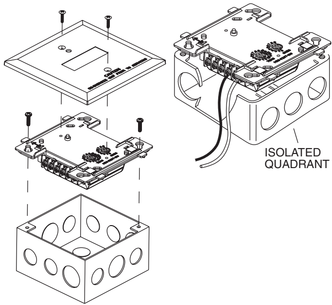
FIGURE 2. MODULE MOUNTING:
