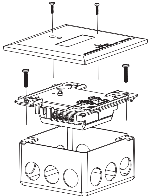
FIGURE 2. MODULE MOUNTING:
